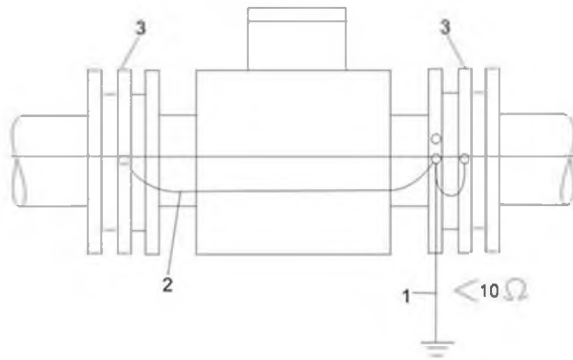
Fig.1 For Mounting to Cathode protected Tubes
